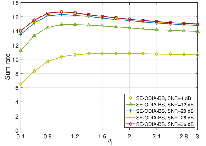
Fig. 2. Sum rate performance of the SE-ODIA-BS versus \eta_I , when K = 3 , M = 4 , S = 2 , L = 2 , N = 40 , and |\mathcal{D}| = 8 .
