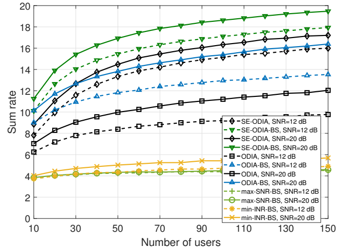
Fig. 3. Sum rate performance of each scheme versus N , when K = 3 , M = 4 , S = 2 , L = 2 , and |\mathcal{D}| = 8 for BS.
